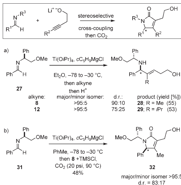
Scheme 2. Stereoselective synthesis of unsaturated 1,5-amino alcohols and tetrasubstituted \alpha,\beta -unsaturated \gamma -lactams.
