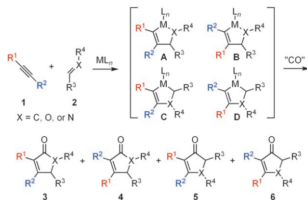
Scheme 1. Regioisomeric products from bimolecular [2+2+1] annulation reactions. L = ligand.
